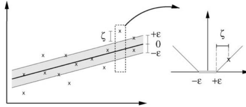
Fig. 2. The soft margin loss setting for linear SVR [8].
