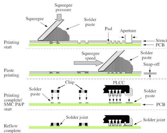
Fig. 1. Main processes of Surface mount technology [1].
