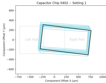
Fig. 6. Behavior of the component positions in P&amp;P process (setting 1 of capacitor chip 0402)
