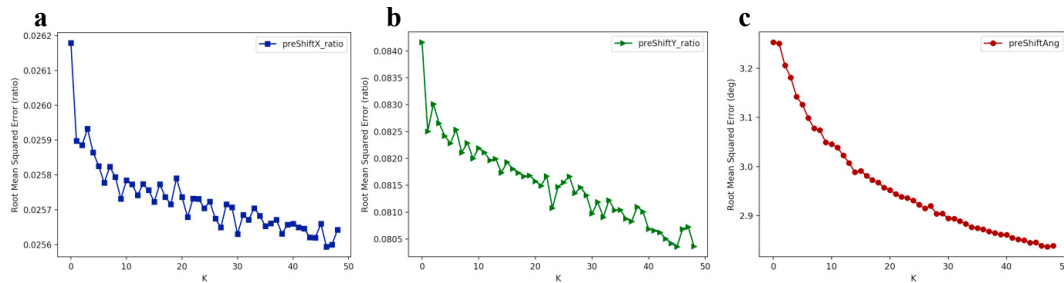
Fig. 8. (a) RMSE across k -fold in x direction; (b) RMSE across k -fold in y direction; (c) RMSE across k -fold in angular direction
