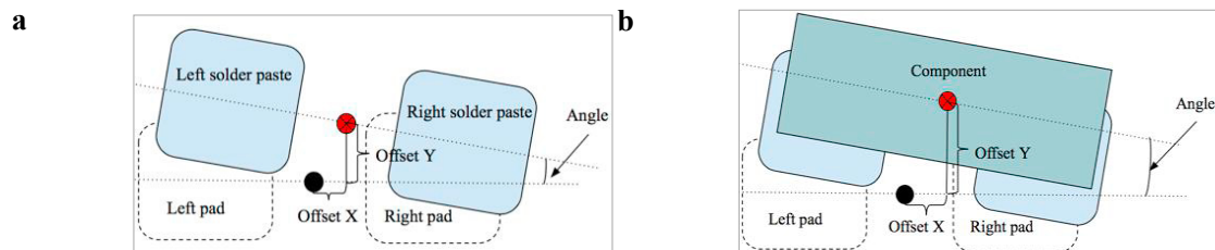
Fig. 5. definition of the offsets: (a) offsets of the solder paste; (b) offsets of the component.
